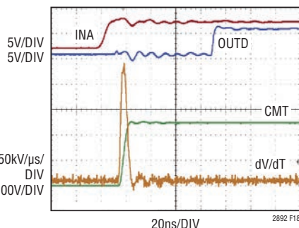
Figure 18. 200kV/ \mu s Transient Prior to Data Transmission
