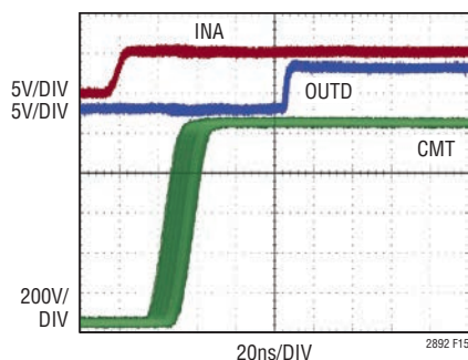
Figure 15. 70kV/ \mu s Transient Operation Coincident with Data Transmission/Reception
