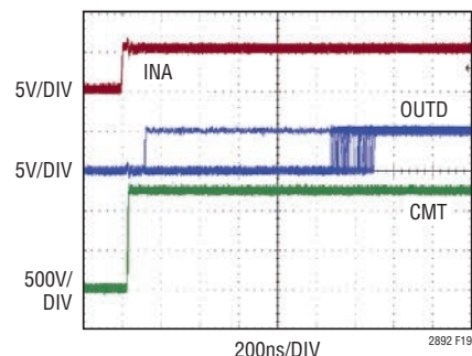
Figure 19. Data Refresh Recovery for 200kV/ \mu s Transient
