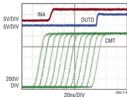
Figure 14. Operation with Repetitive Bursts of Common Mode Transients, 50kV/ \mu s
