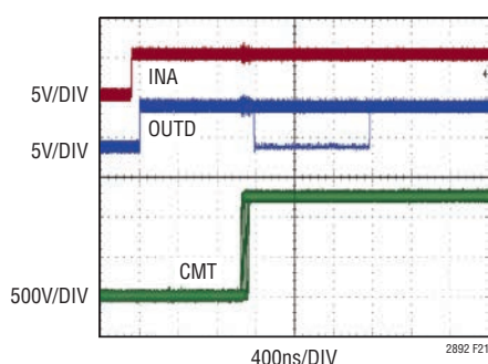
Figure 21. Common Mode Transient (200kV/ \mu s) Coincident with Data Refresh, Data High
