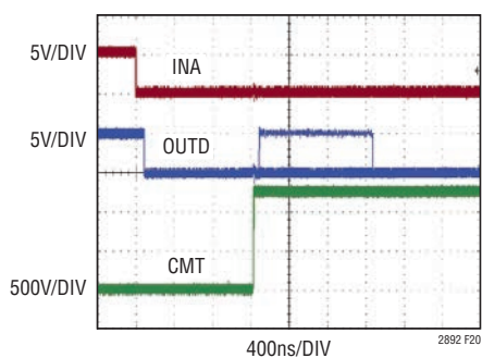
Figure 20. Common Mode Transient (200kV/ \mu s) Coincident with Data Refresh, Data Low
