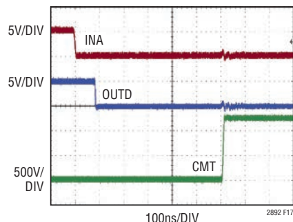
Figure 17. Static Operation with 200kV/ \mu s Transients
