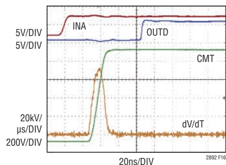
Figure 16. Transient dV/dT, 70kV/ \mu s
