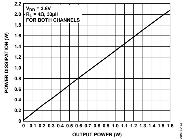
Figure 24. Power Dissipation vs. Output Power at V_{DD} = 3.6\text{ V} , R_L = 4\ \Omega
