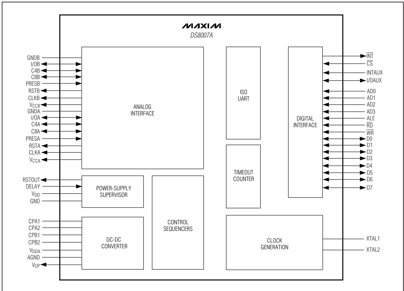
Figure 6. Block Diagram
