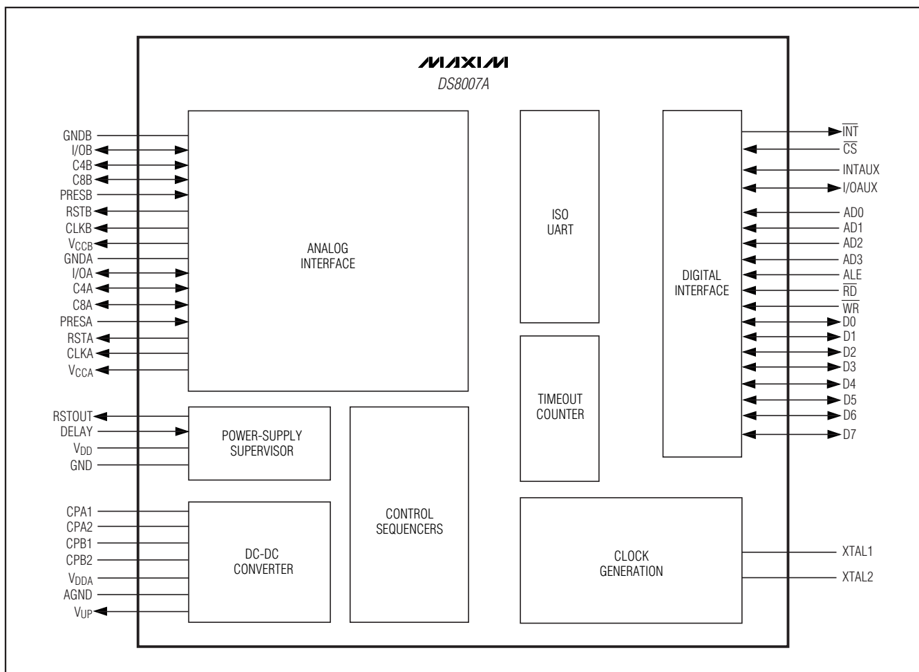
Figure 6. Block Diagram
