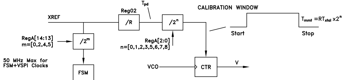
Figure 41. VCO Calibration
