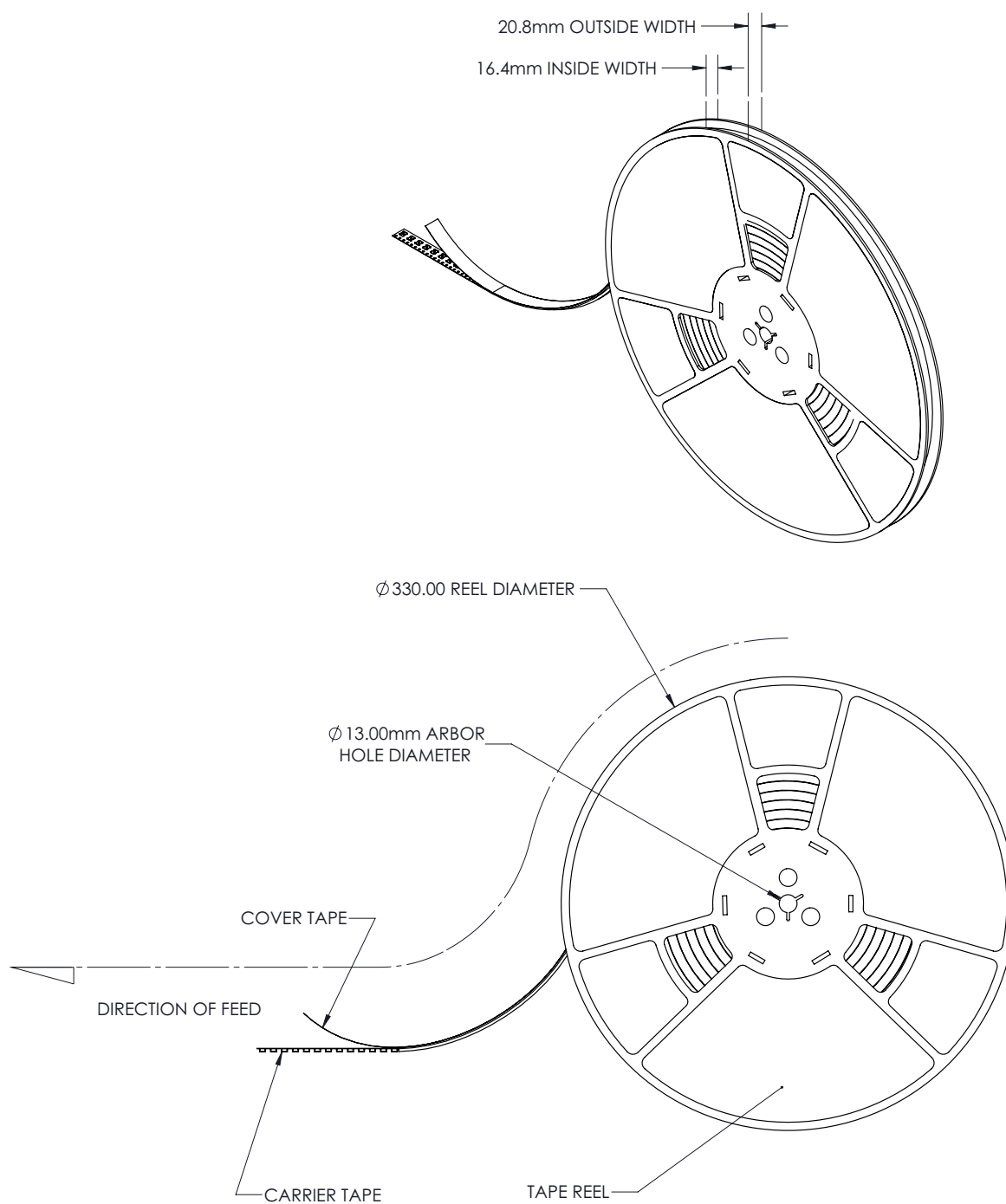
Figure 13. Reel dimensions for LUXEON MX.
