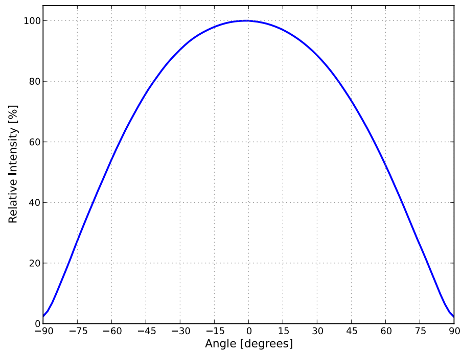
Figure 6. Typical radiation pattern for L1MX-xxxxxxxxxx0 at specified test current, T_j = 85^\circ\text{C} .
