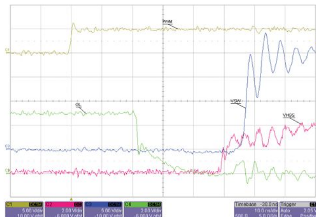
Switching Waveform at PWM Rising Edge V_{IN} = 19\text{ V} , V_O = 1.8\text{ V} , I_O = 20\text{ A} , f_{SW} = 500\text{ kHz}
