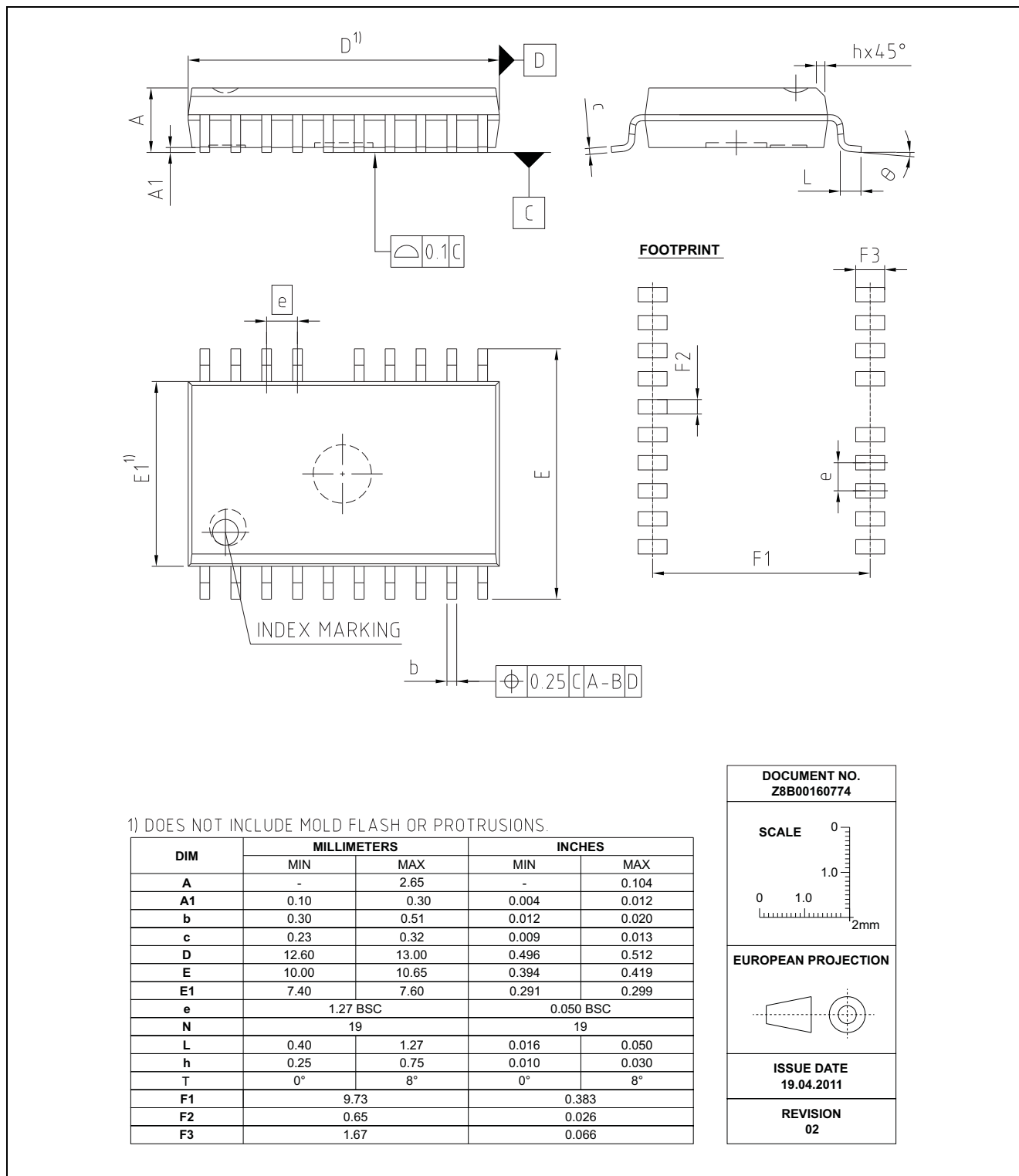
Figure 9 PG-DSO-19-4
