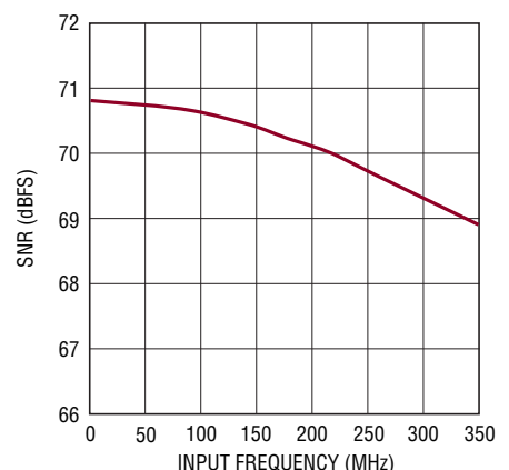
LTC2175-12: SNR vs Input Frequency, -1dB, 2V Range, 125Mps
