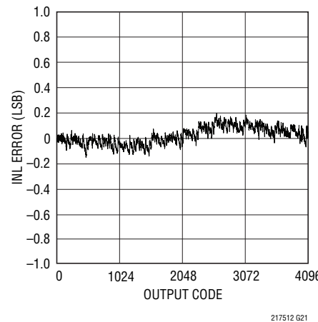
LTC2174-12: Integral Nonlinearity (INL)
