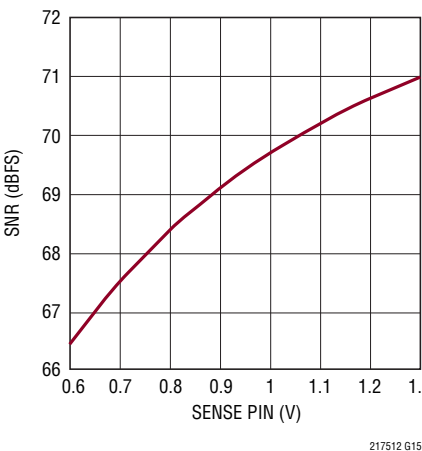
LTC2175-12: SNR vs SENSE, f_{IN} = 5\text{MHz} , -1dB
