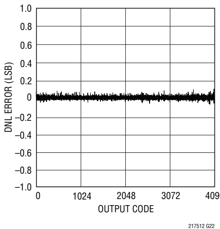
LTC2174-12: Differential Nonlinearity (DNL)
