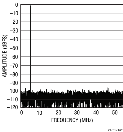
LTC2174-12: 8k Point FFT, f_{IN} = 5\text{MHz} , -1dBFS, 105Msps
