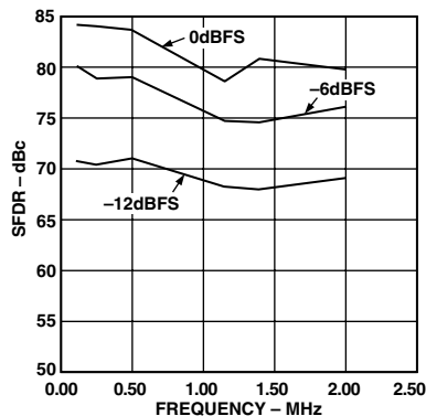
Figure 22. SFDR vs. f_{OUT} @ 5 MSPS
