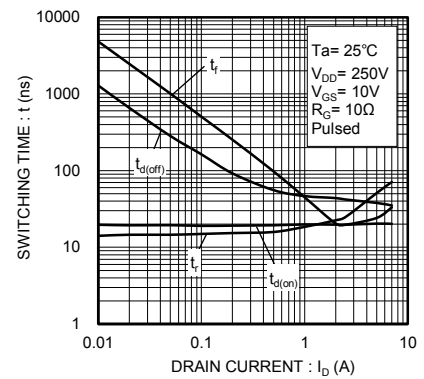
Fig.12 Switching Characteristics
