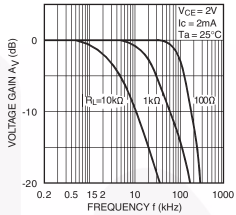
Fig. 14 Frequency Response
