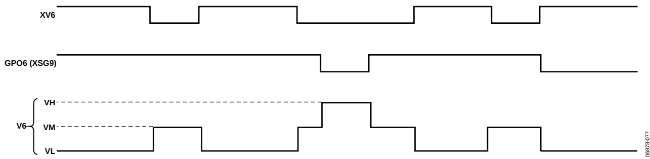
Figure 77. XV6, GPO6, and V6 Output Polarities ( \overline{\text{LEGEN}} = High)
