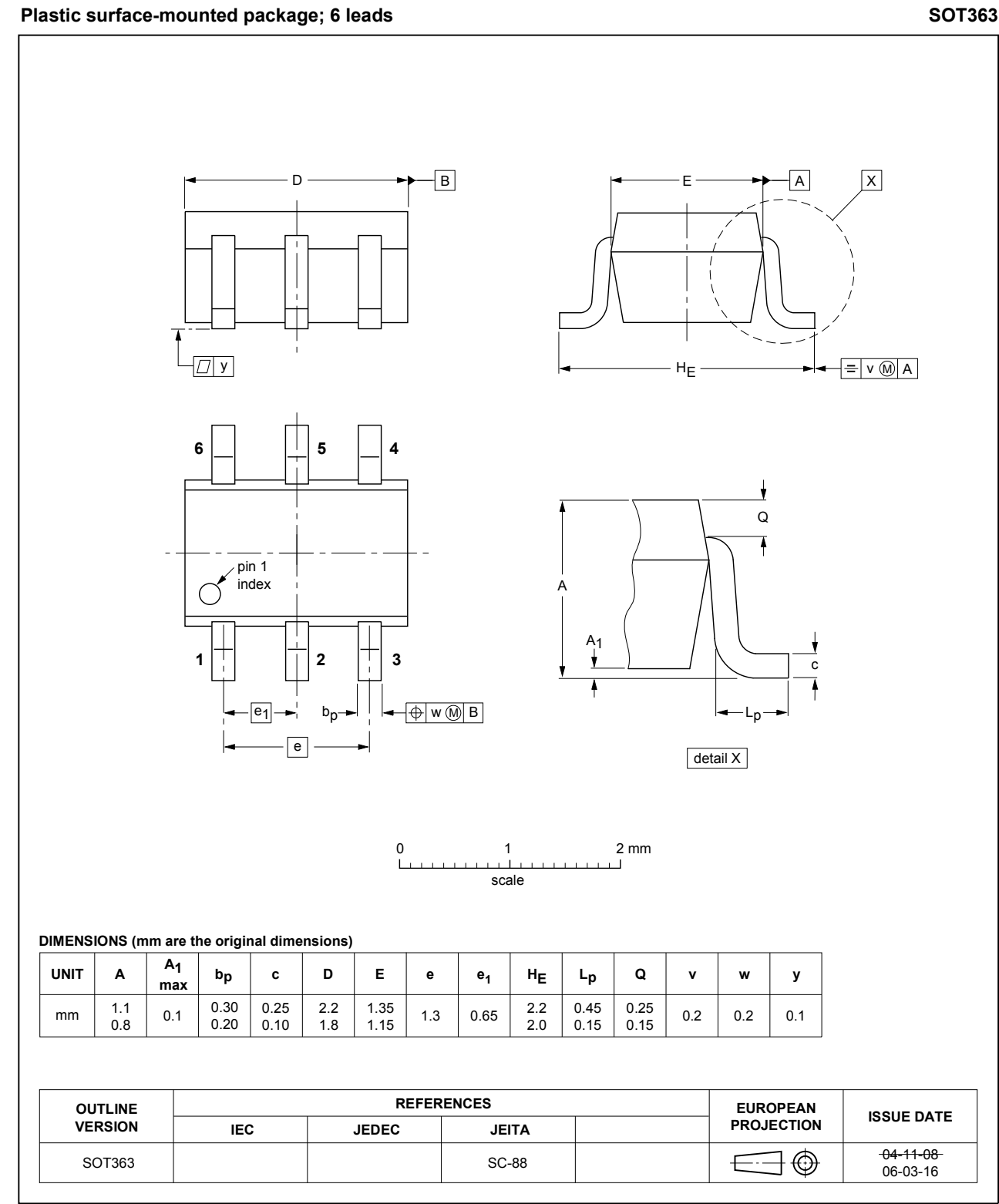
Fig. 8. Package outline SOT363 (SC-88)
