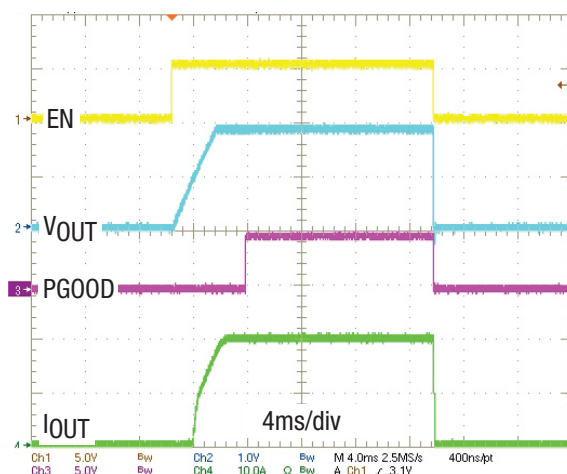
Figure 14. Enable Functionality, V_{IN} = 12V
