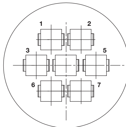
Arrangement 23-7 Max. Wire Ins. Dia. = .220 [5.59]
