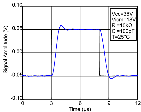
Figure 21: Small step response vs. time at V_{CC} = 36\text{ V}
