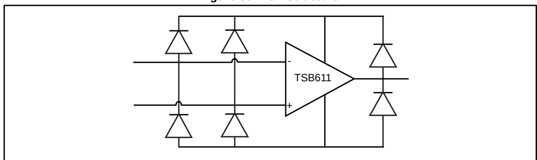
Figure 35: ESD structure
