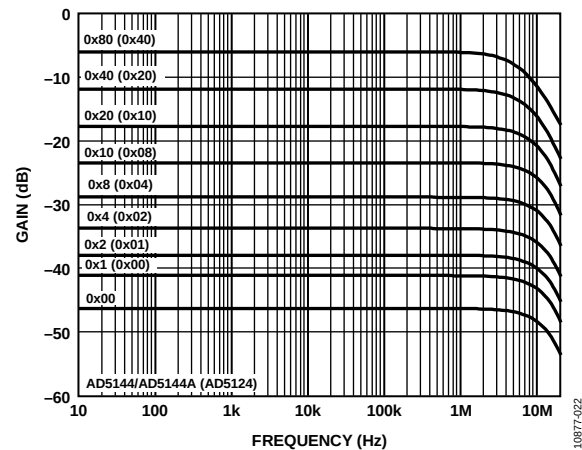
Figure 25. 10 kΩ Gain vs. Frequency vs. Code
