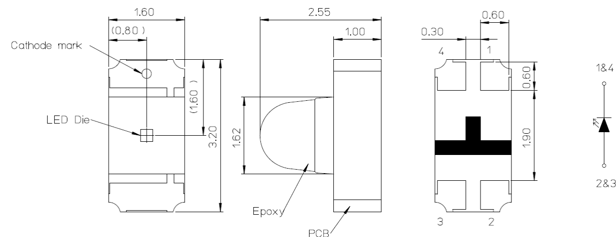
Figure 1: Package Dimensions
