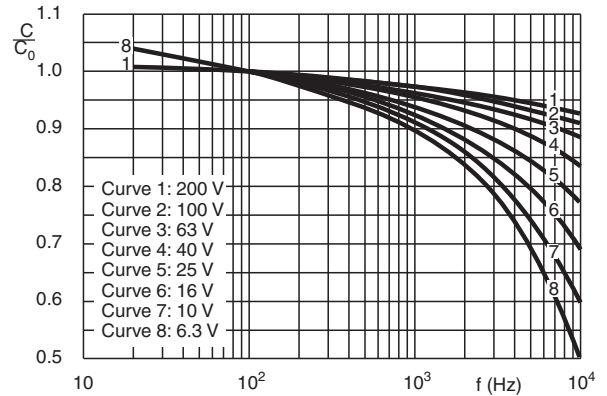
Case Ø D x L = 10 mm x 30 mm to 21 mm x 38 mm C_0 = Capacitance at 20 °C, 100 Hz
