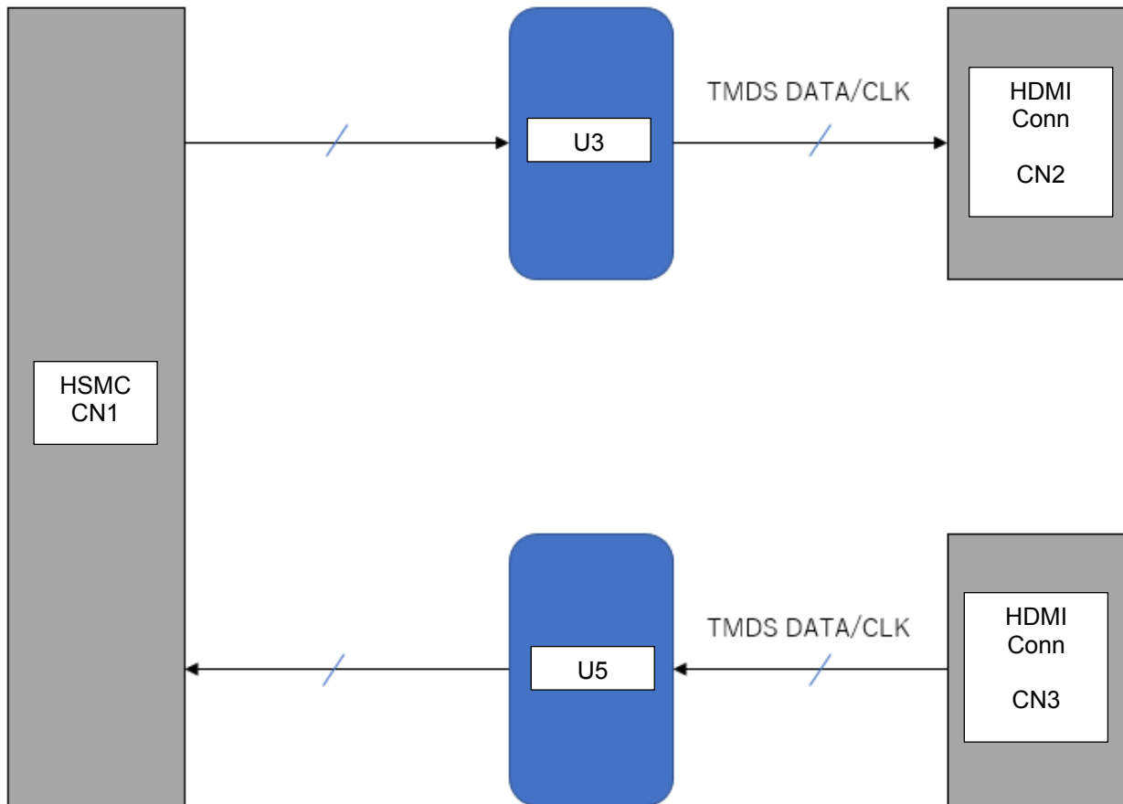
Figure 4-1. Block Diagram
