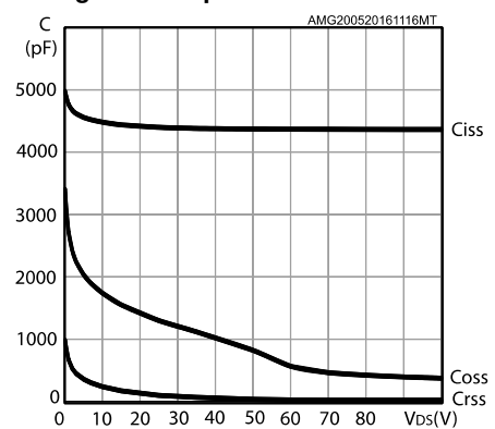
Figure 9: Capacitance variations
