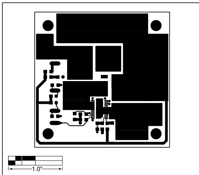
Figure 3. MAX1709 EV Kit PC Board Layout—Component Side
