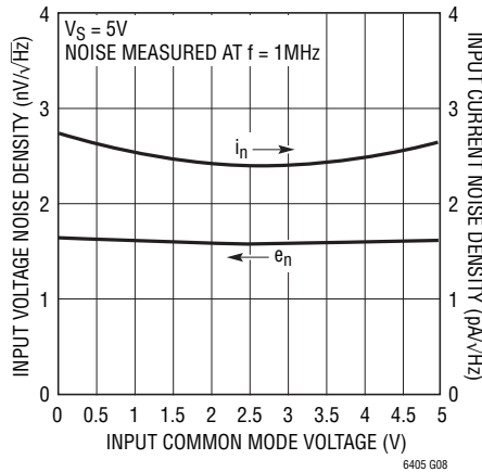
Input Noise Density vs Input Common Mode Voltage
