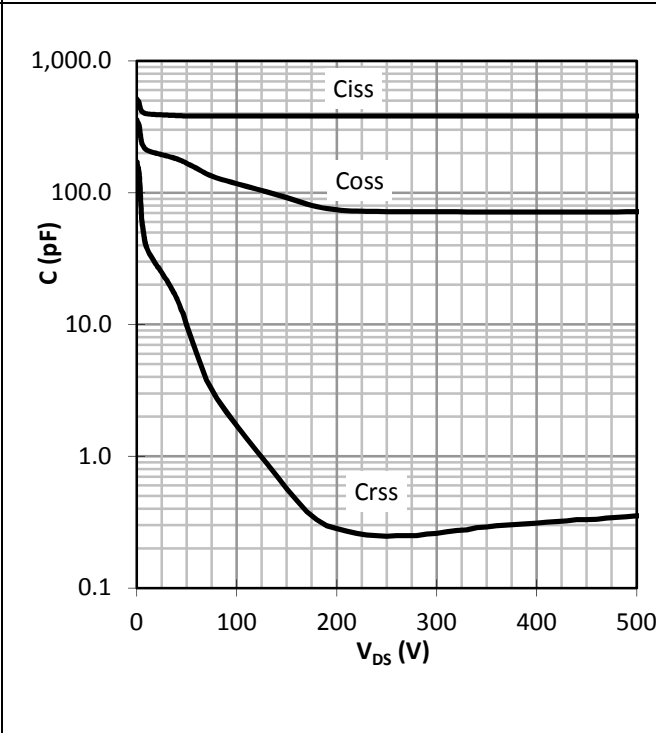
Figure 20 Typ. capacitances
