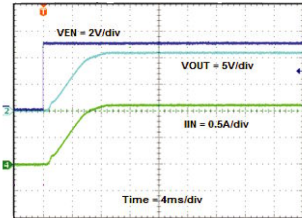
Figure 21 - Turn On Time, V_{IN} = 12\text{ V} , C_{SS} = 47\text{ nF} , R_L = 10\ \Omega , C_L = 10\ \mu\text{F}
