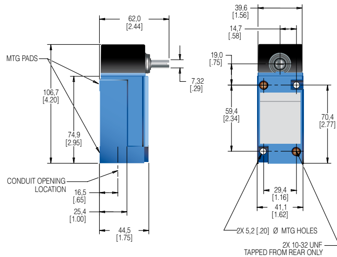
SPDT Plug-in (mm[in])
