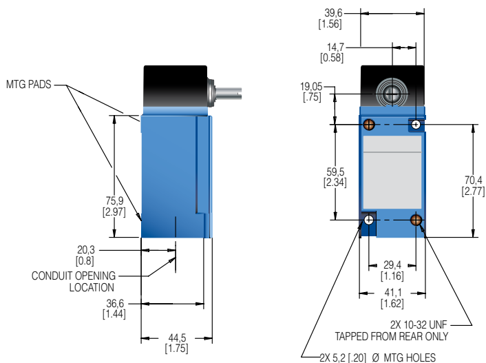
SPDT Non-plug-in (mm[in])
