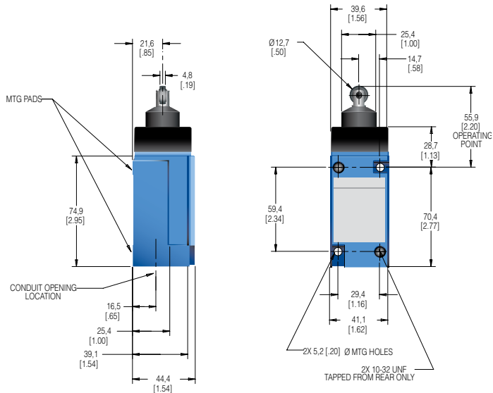
SPDT Non-plug-in (mm[in])
