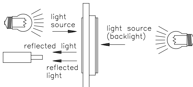
Transmissive Type
