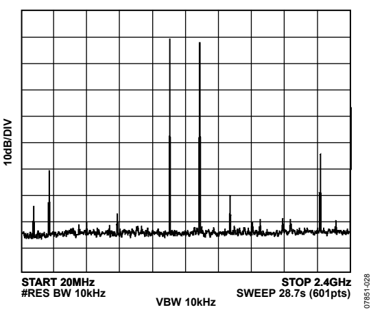
Figure 28. Single-Tone Spectrum in Mix Mode at f_{OUT} = 1.31 \text{ GHz} , f_{DAC} = 2.4 \text{ GSPS}
