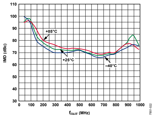
Figure 22. IMD vs. f_{OUT} over Temperature
