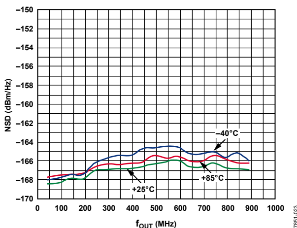
Figure 23. Eight-Tone NSD vs. f_{OUT} over Temperature
