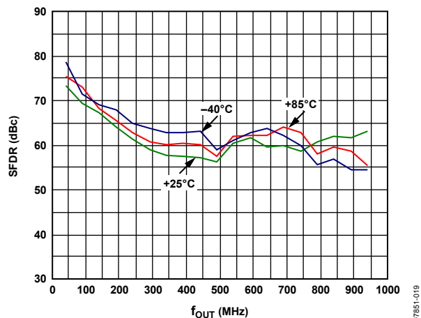
Figure 19. SFDR vs. f_{OUT} over Temperature
