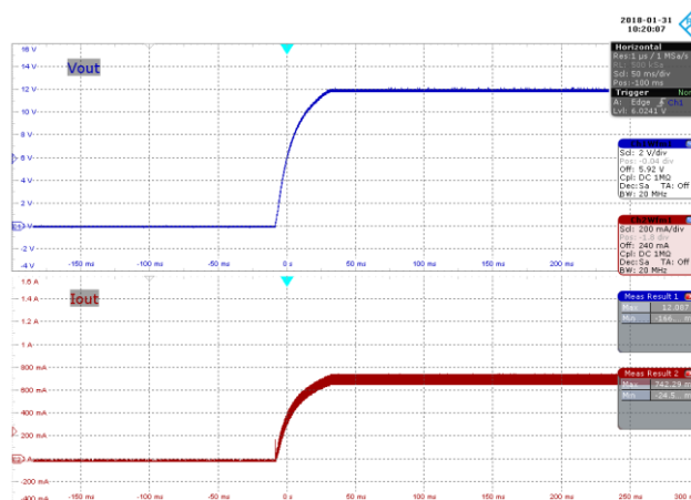
Figure 53 – 115 VAC 60 Hz, Full Load Start-up. Upper: V_{OUT} , 2 V / div., 50 ms / div. Lower: I_{OUT} , 200 mA / div., 50 ms / div.
