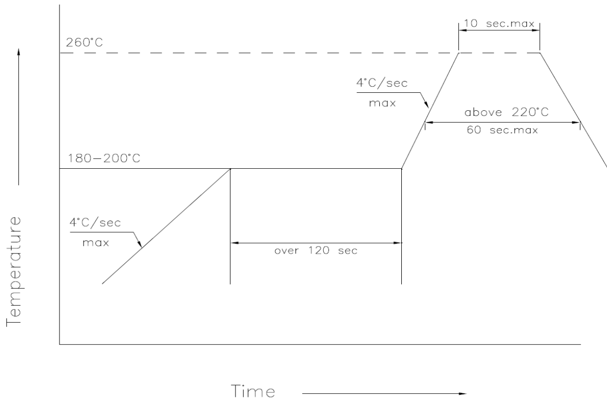
Figure 7: Reflow soldering profile
