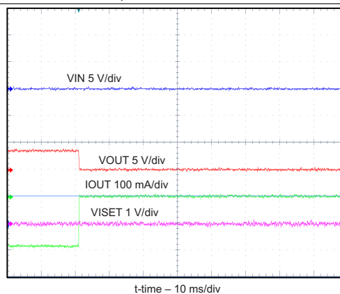
Figure 12. Battery Removal
