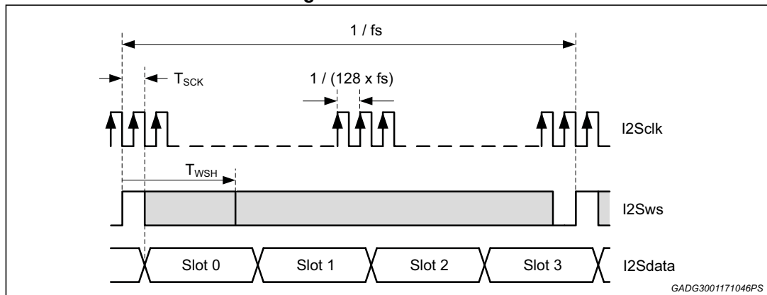
Figure 65. TDM4 mode
