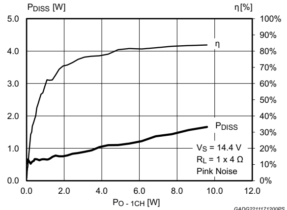
Figure 5. Efficiency and power dissipation ( V_S = 14.4\text{ V} , R_L = 1 \times 4\ \Omega , f = 1\text{ kHz} pink noise)
