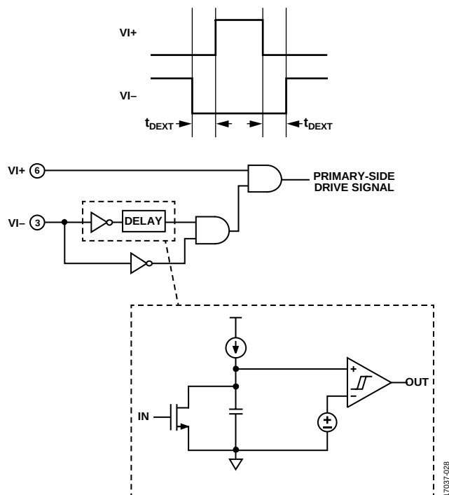
Figure 28. Dead Time Control
