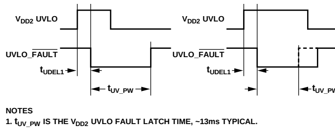
Figure 26. \overline{\text{UVLO\_FAULT}} Fault for V_{\text{DD2}} UVLO
