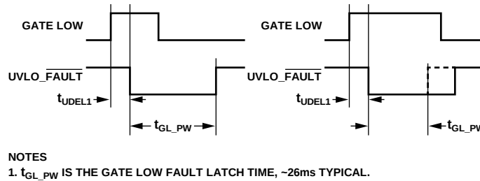
Figure 27. \overline{\text{UVLO\_FAULT}} Fault, Gate Low
