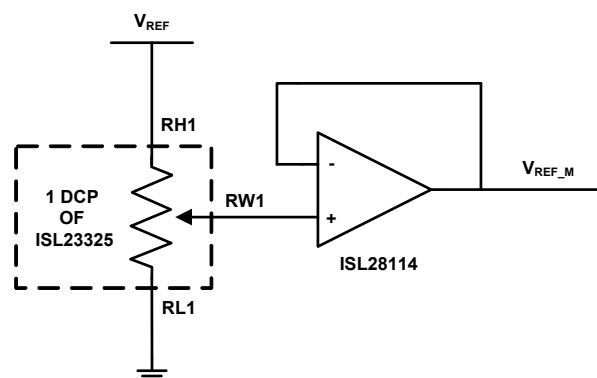
FIGURE 2. V_{\text{REF}} ADJUSTMENT
