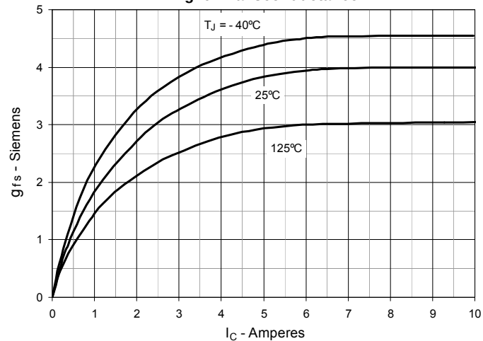
Fig. 6. Transconductance
