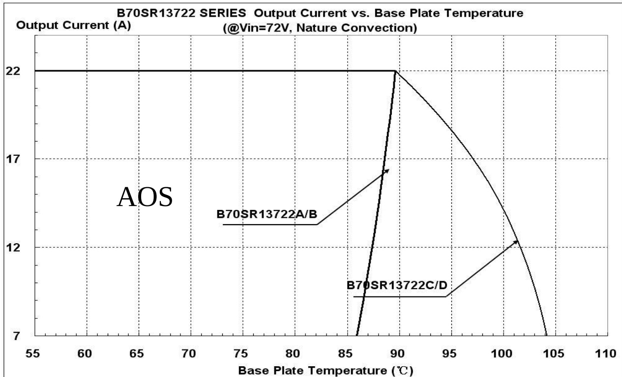
Figure 22: Output Current vs. base plate temperature @Vin=72V
