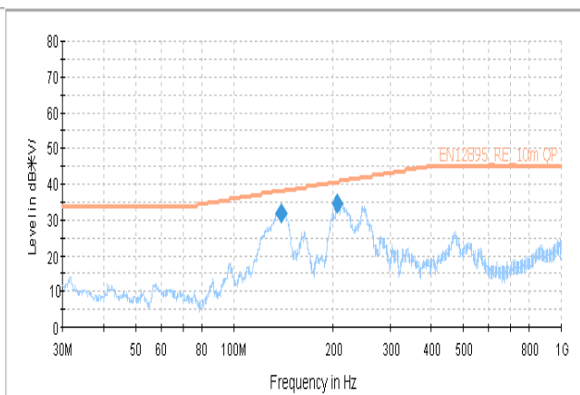
Figure 15: test result(Horizontal)
