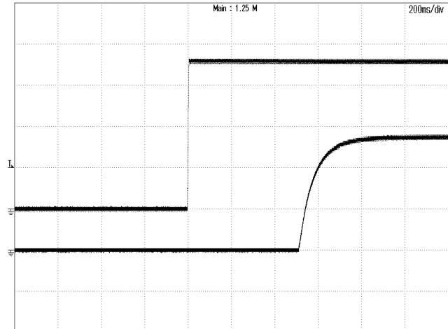
Figure 4: Vout start up with Vin on at 72Vin, 22A lout, TOP: VIN, 20V/div, 200mS/div BOTTOM: VOUT, 5V/div, 200mS/div
