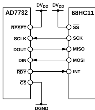
Figure 13. AD7732 to Host Device Interface, SPI
