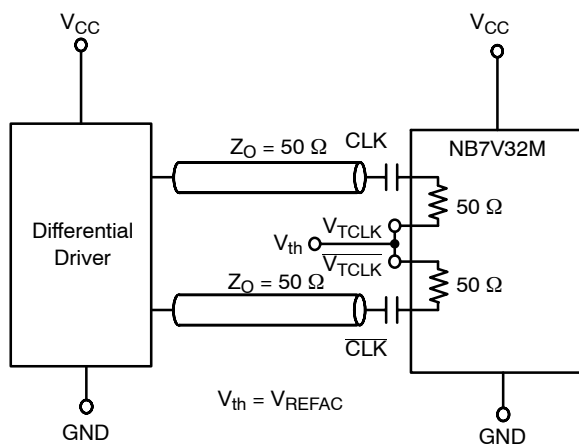
Figure 15. Capacitor-Coupled Differential Interface ( \sqrt{V_{TCLK}/V_{TCLK}} Connected to V_{REFAC} ; V_{REFAC} Bypassed to Ground with 0.1 \mu F Capacitor)
