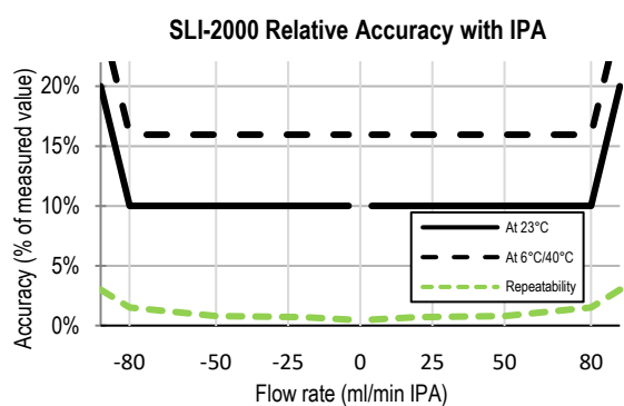
Figure 2: Flow meter accuracy and repeatability across the flow range. Relative error in % of measured value (left column) and absolute error in \mu\text{l/min} or \text{ml/min} in case of the SLI-2000 (right column) for IPA
