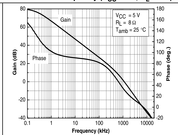
Figure 10. Open loop gain and phase vs. frequency ( V_{CC} = 5\text{ V} , R_L = 8\ \Omega )
