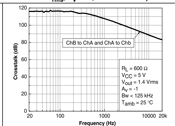
Figure 36. Crosstalk vs. frequency (R_L = 600\ \Omega, V_{CC} = 5\ \text{V}, V_{out} = 1.4 V_{rms}, A_V = -1, BW < 125\ \text{kHz})
