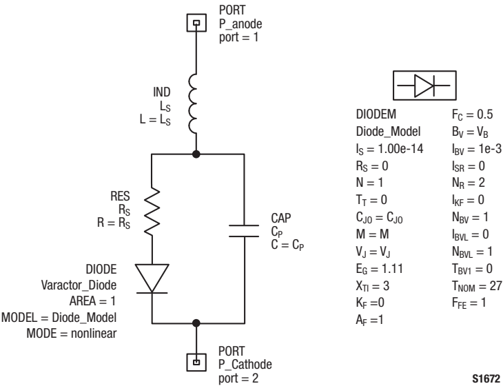
Figure 3. SPICE Model
