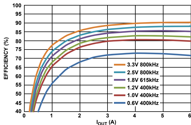
FIGURE 13. ZL9006M EFFICIENCY, V_{IN} = 12V
