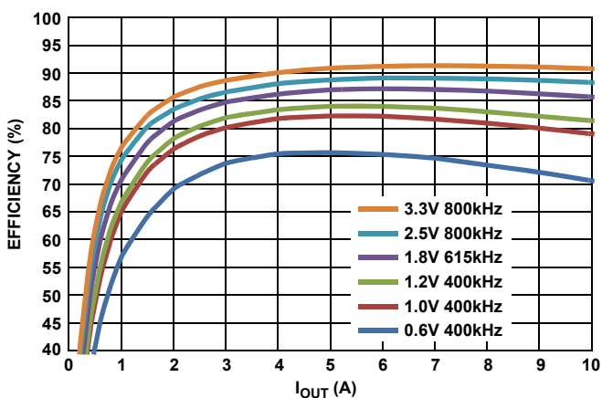
FIGURE 15. ZL9010M EFFICIENCY, V_{IN} = 12V
