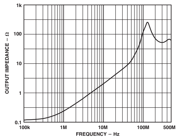
TPC 24. AD8111 Output Impedance, Enabled
