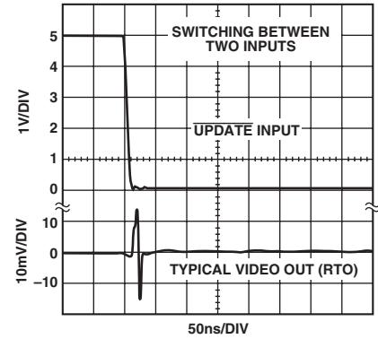
TPC 22. AD8111 Switching Transient (Glitch)
