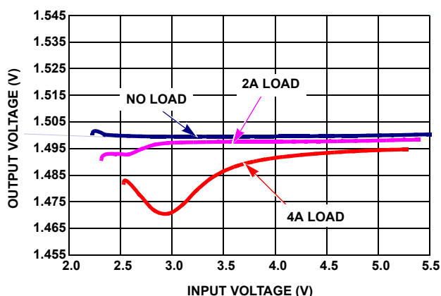
FIGURE 13. V_{OUT1} = 1.5V REGULATION vs V_{IN}
